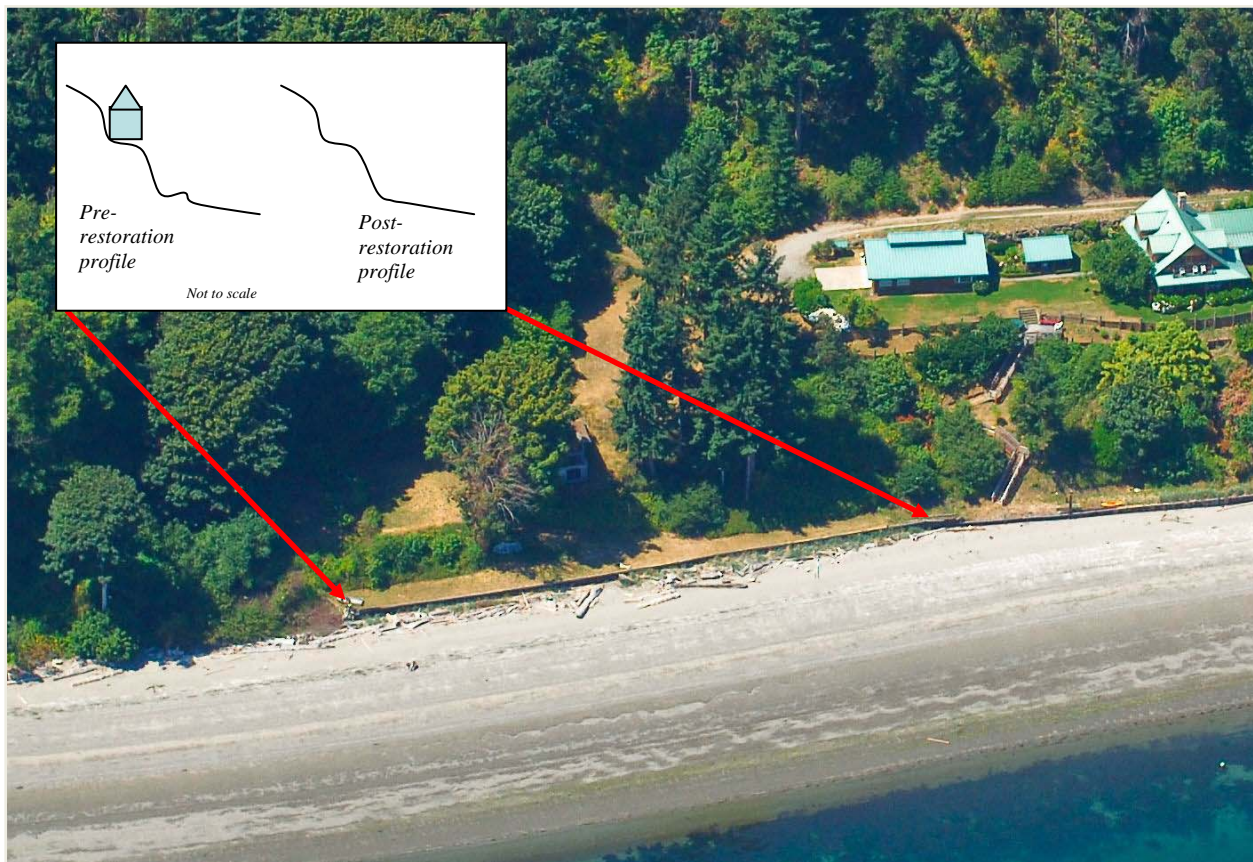
Figure 12 Oblique image of Piner Point project site (2006) with an example cross section of the project site before and after the restoration project.
